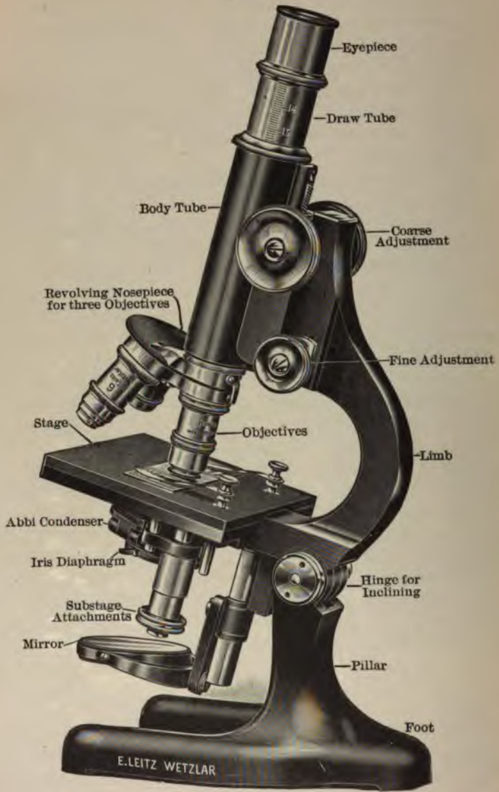
FIG. 8.—Compound Microscope
