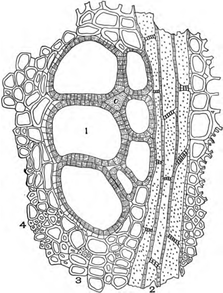
CROSS-SECTION OF QUASSIA WOOD ( Picrana excelsa [Sw.], Lindl.)
