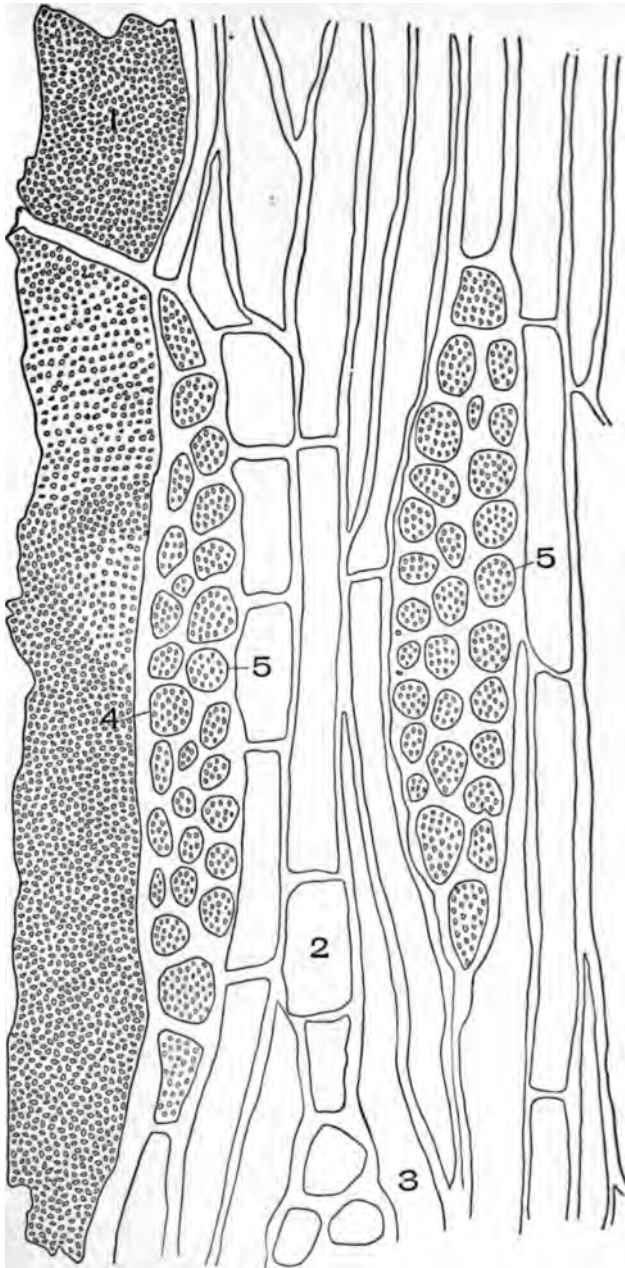
TANGENTIAL SECTION OF QUASSIA WOOD ( Picramnia excelsa [Sw.], Lindl.) 1. Vessel. 2. Wood parenchyma. 3. Wood fibre. 4. End wall of medullary ray cell. 5. Medullary ray bundle.
