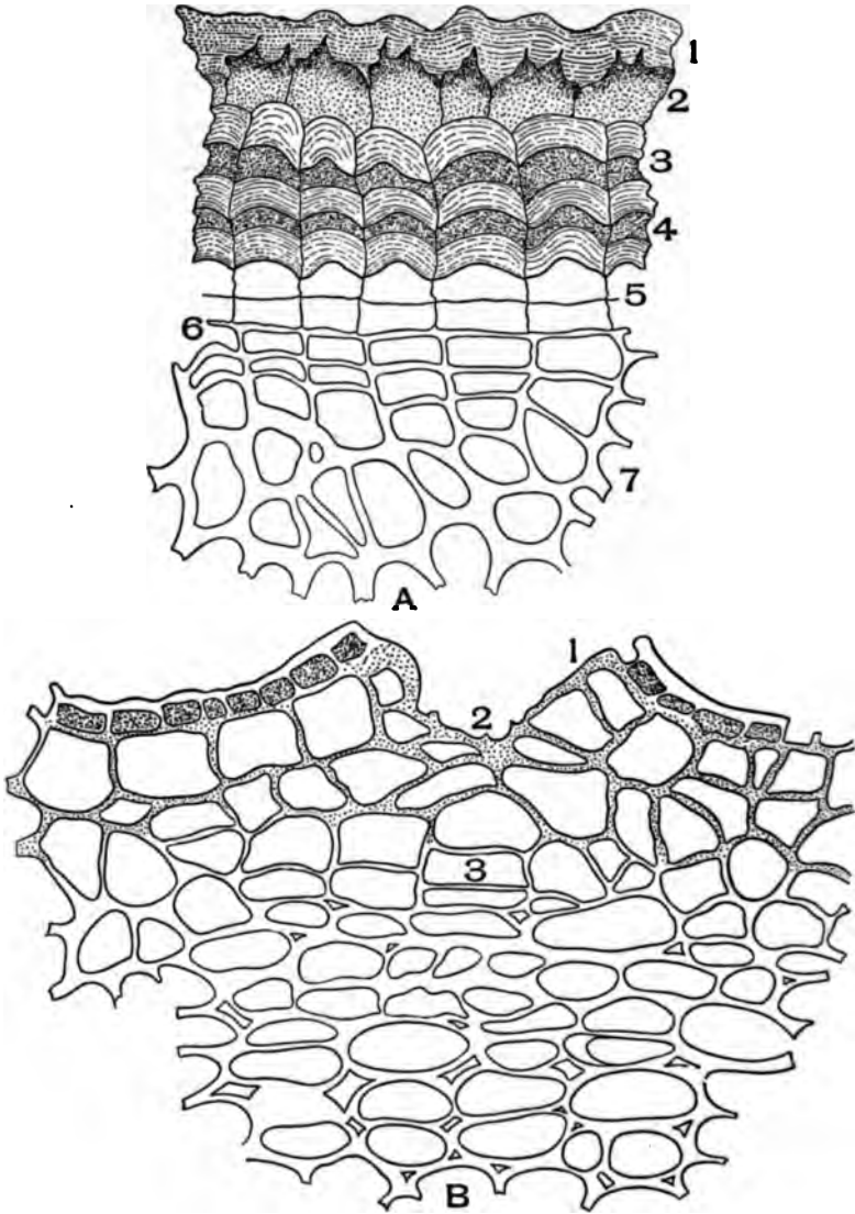
A. Cross-section of buchu stem ( Barosma betulina [Berg.], Barth. and Wendl.). 1, Outer wall of epidermis; 2, Cell cavity of epidermal cell; 3, Wall of cork cell; 4, Cavity of cork cell; 5, Phellogen layer; 6, Divided phellogen cell changing into a cortical parenchyma cell; 7, Cortical parenchyma cell. B. Cross-section of leptandra rhizome ( Leptandra virginica [L.], Nutt.). 1, Parenchyma cells undergoing change in the composition of their walls; 2, A break in the epidermal tissue; 3, Parenchyma cells undergoing division.
