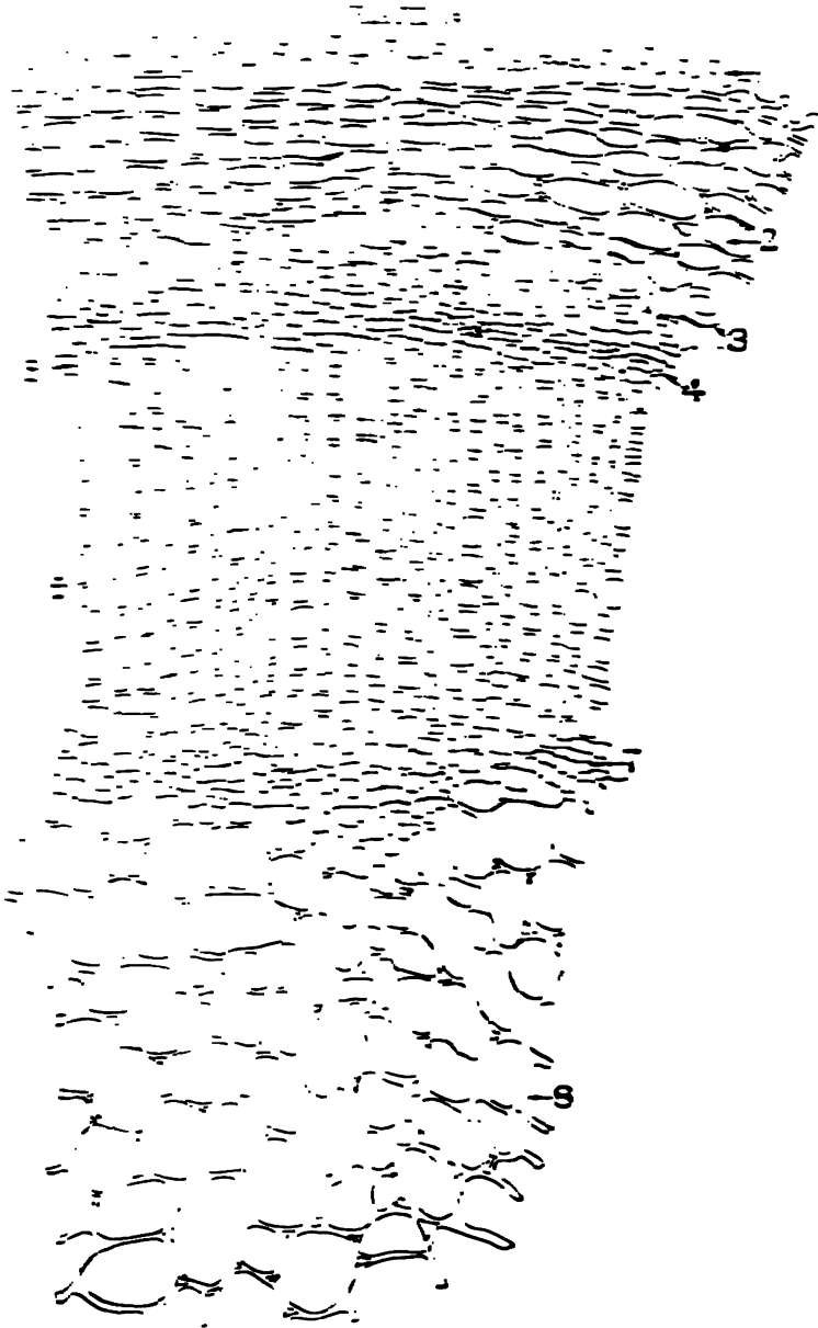
CROSS-SECTION OF STEM OF SPIGELLA MARYLANDICA, L.
