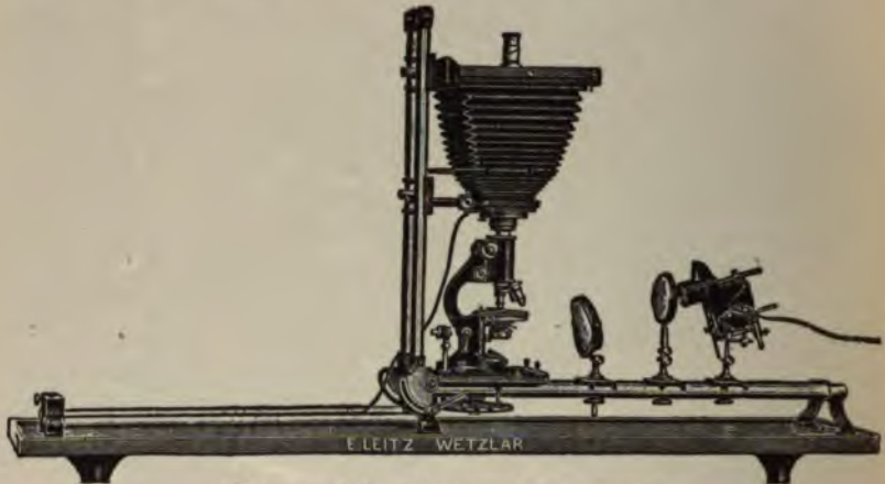
FIG. 29.—Microphotographic Apparatus
